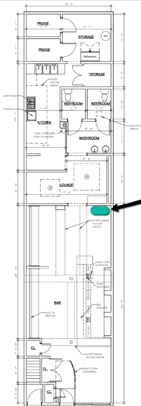
1 EXISTING FIRST FLOOR PLAN 1/4" = 1'-0"
