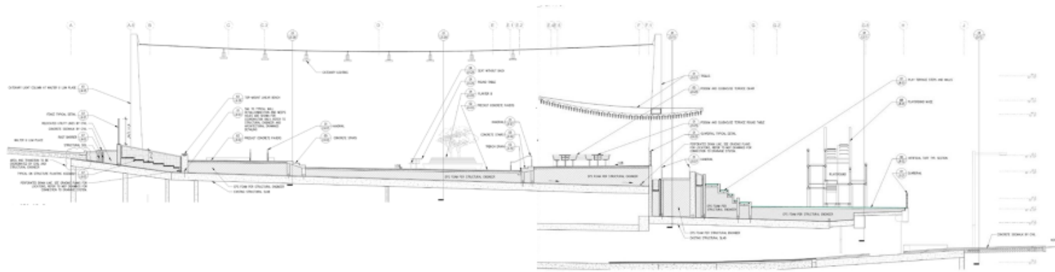
SEC 02 UPPER PLAZA AND LOWER PLAYGROUND SECTION
